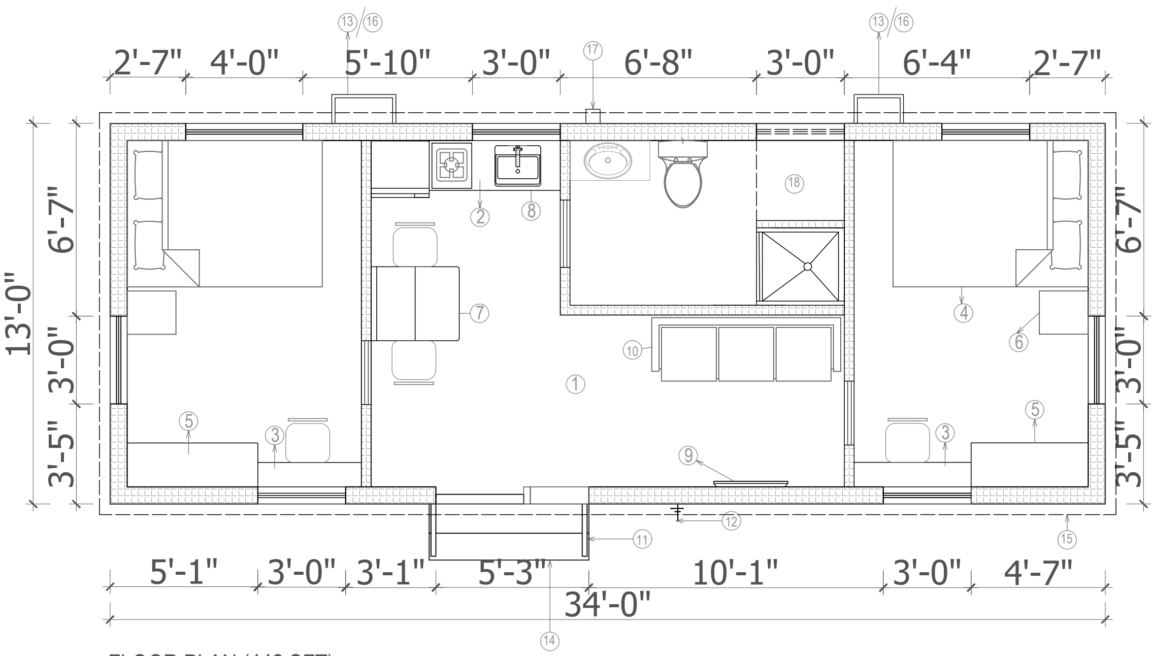
FLOOR PLAN (442 SFT)
