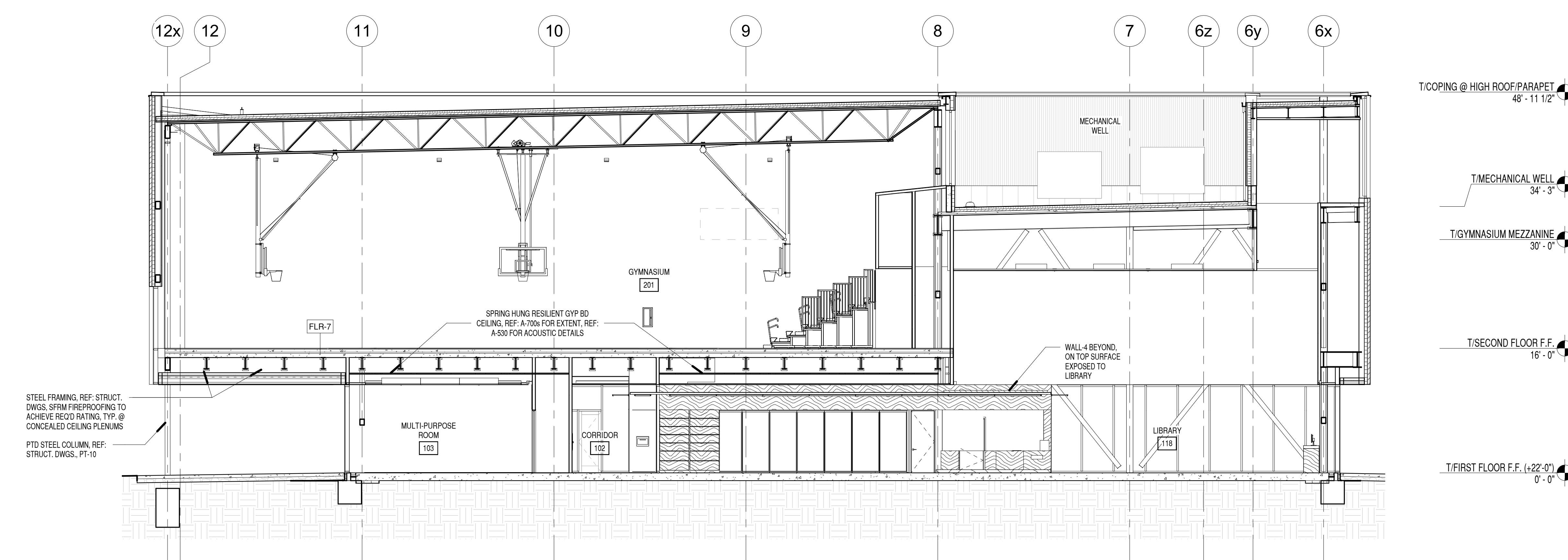
1 east/west section A350 SCALE: 1/8" = 1'-0"
