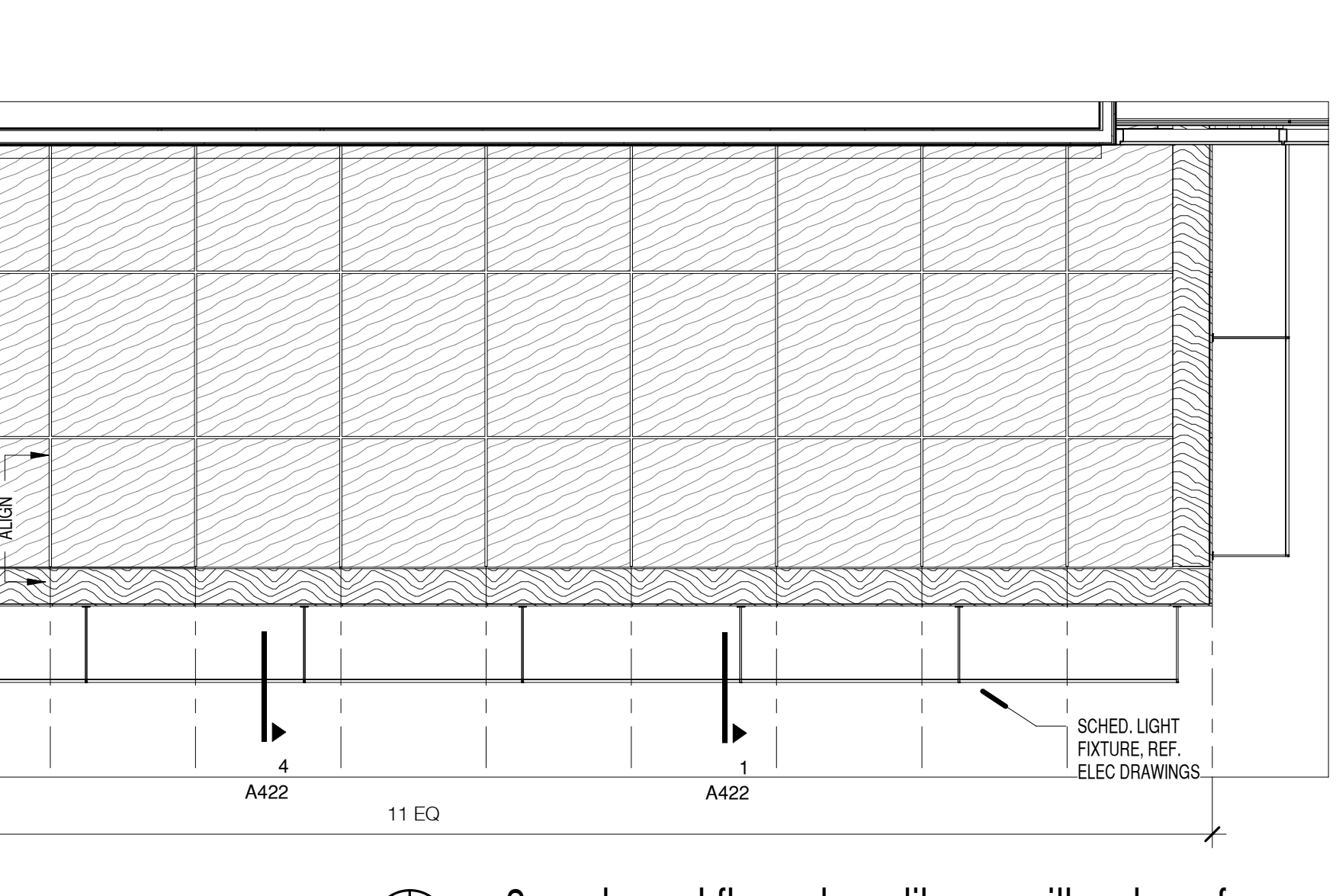
3 enlarged floor plan - library millwork roof A102.1 SCALE: 1/4" = 1'-0"
