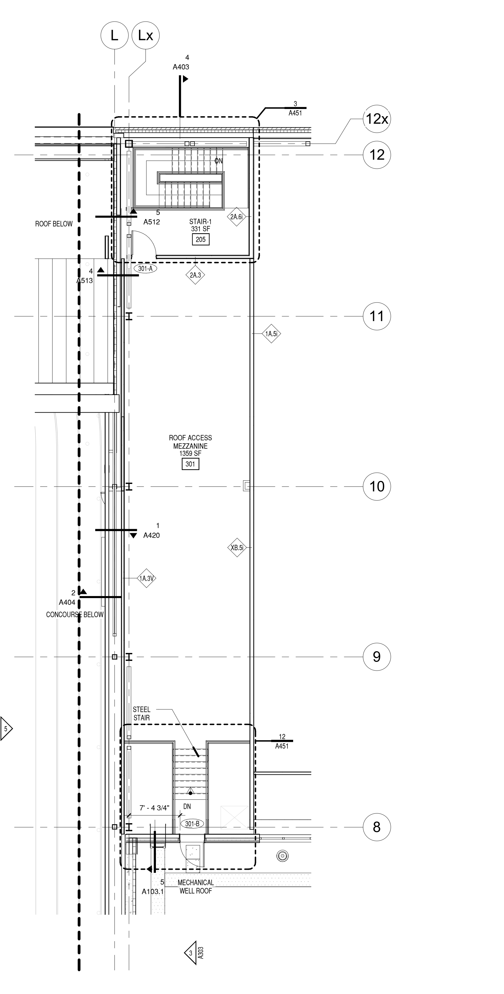
2 gymnasium mezzanine plan A102.1 SCALE: 1/8" = 1'-0"
