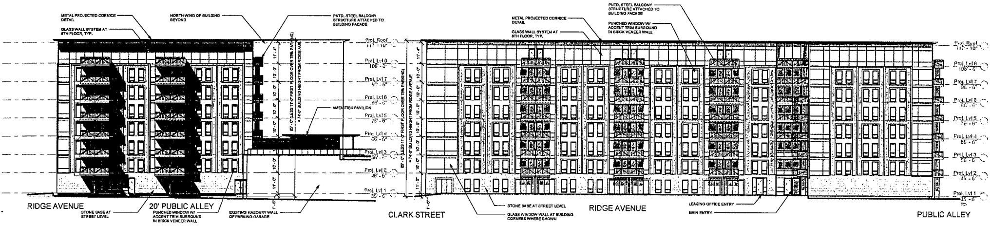
4 SOUTH ELEVATION 0 4 8 16 32
