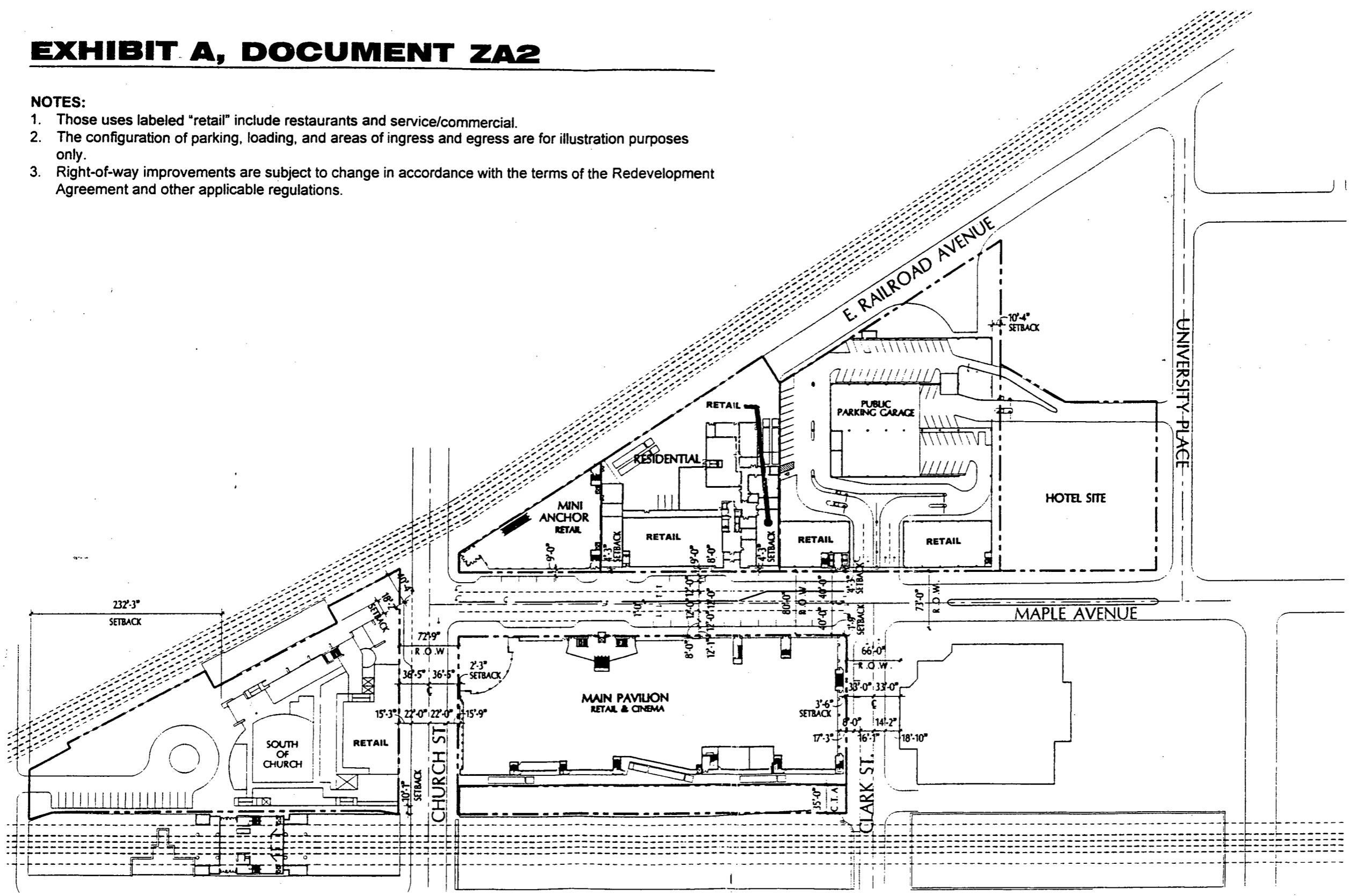
1 SITE PLAN 1"=50'-0"
