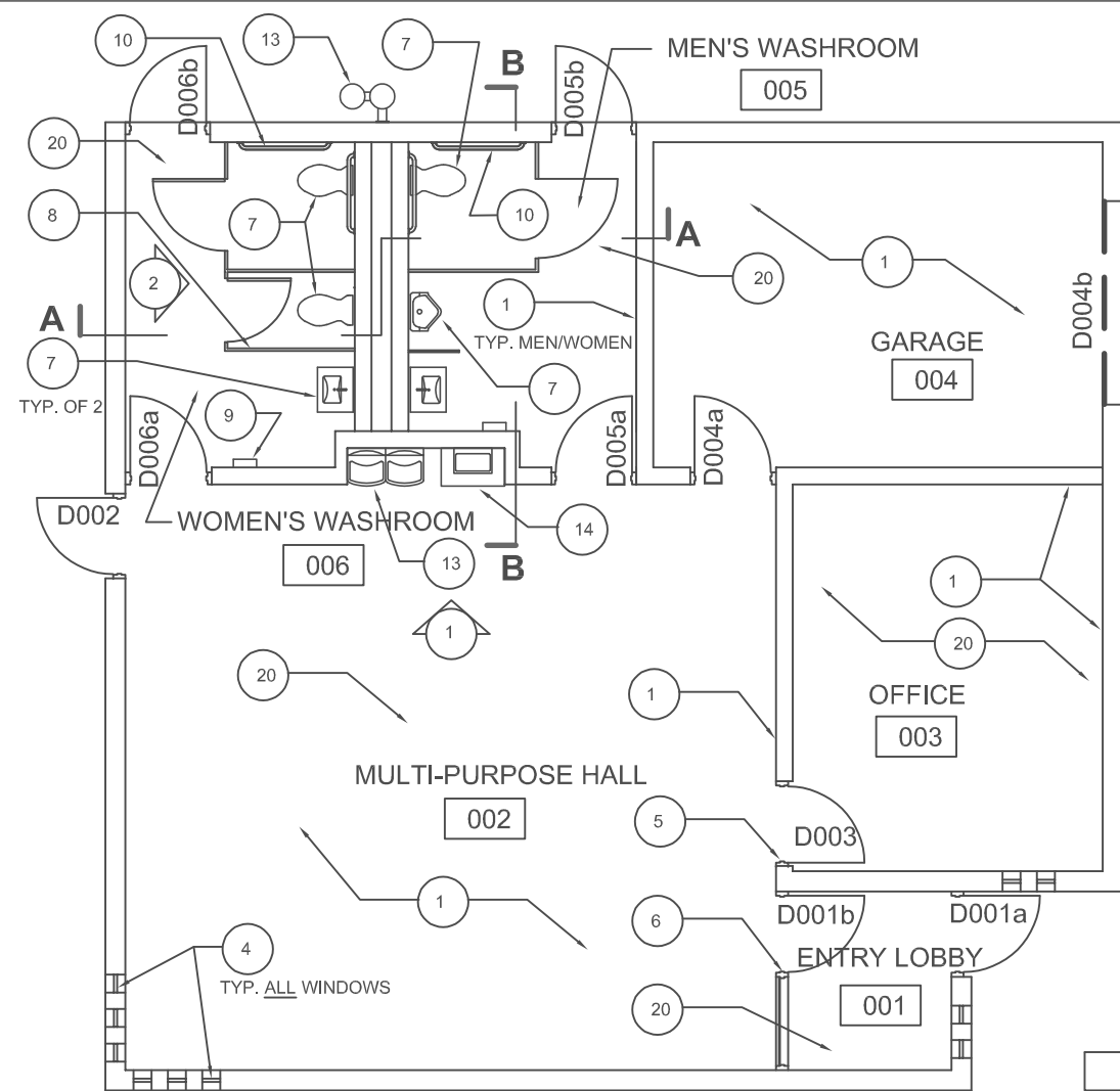
FLOOR PLAN
