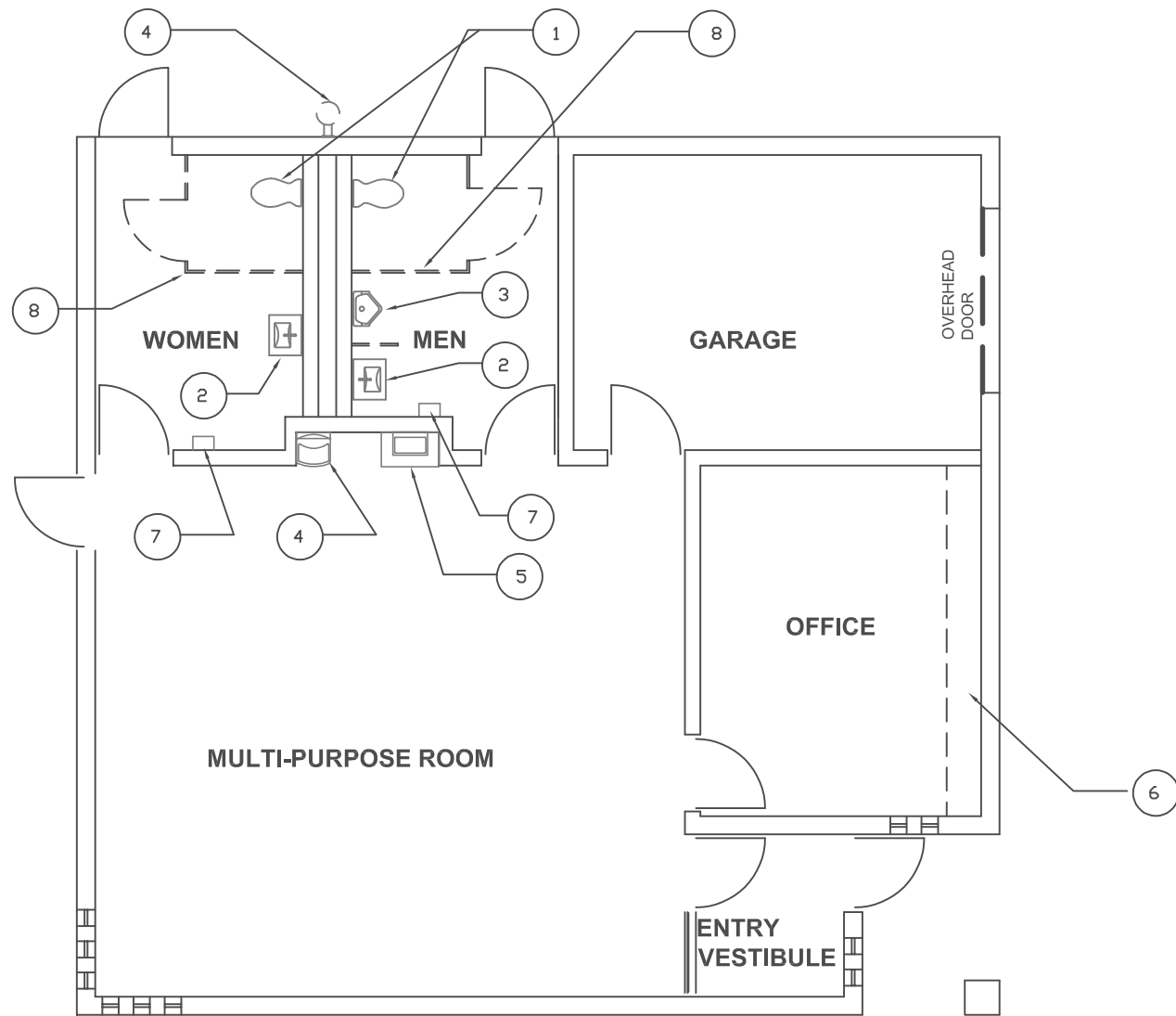
DEMOLITION PLAN
